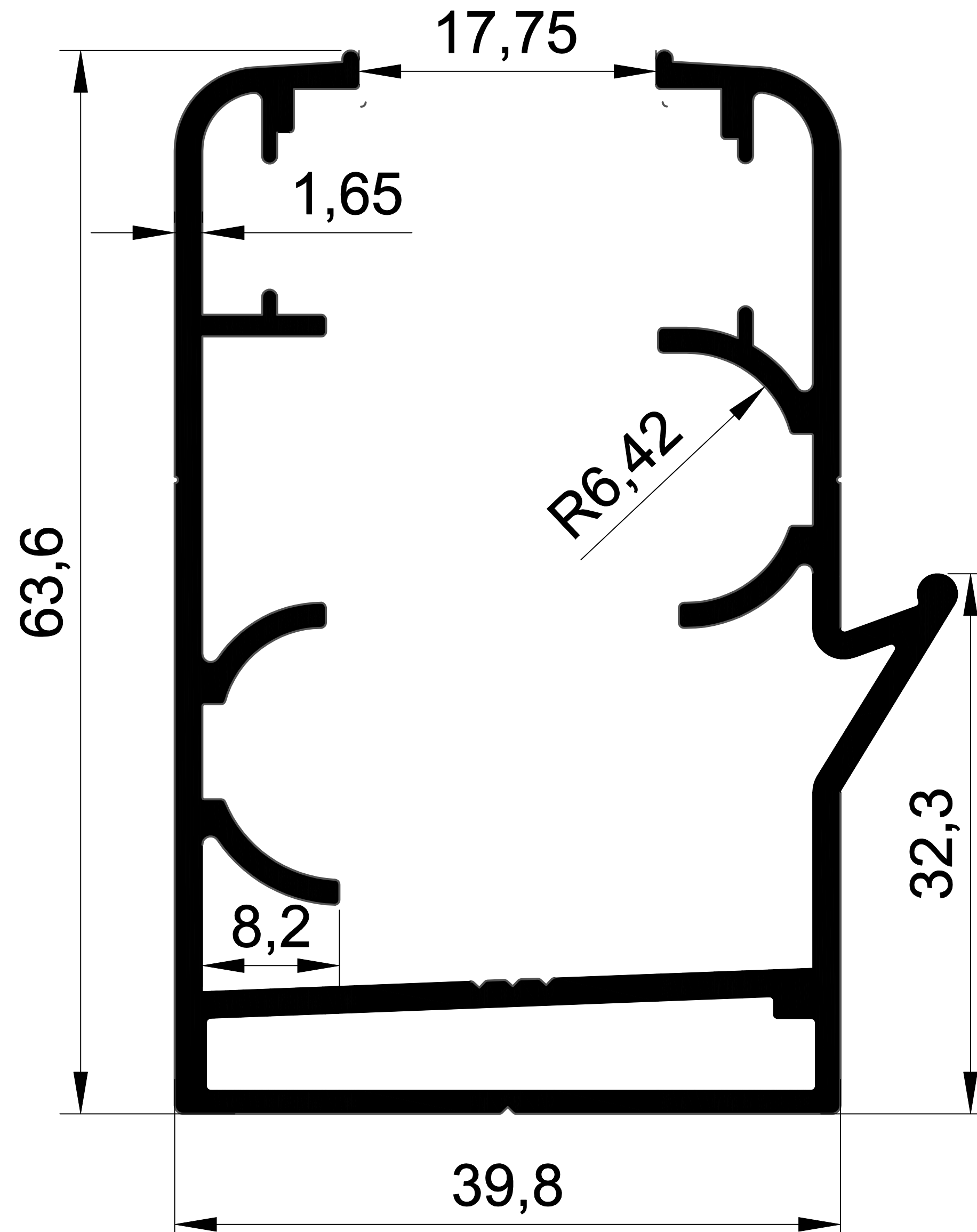
EKOL 1456 1,222 gr/m. GOLD ORTADAN DAMLALIKLI KASA-1.65 mm
