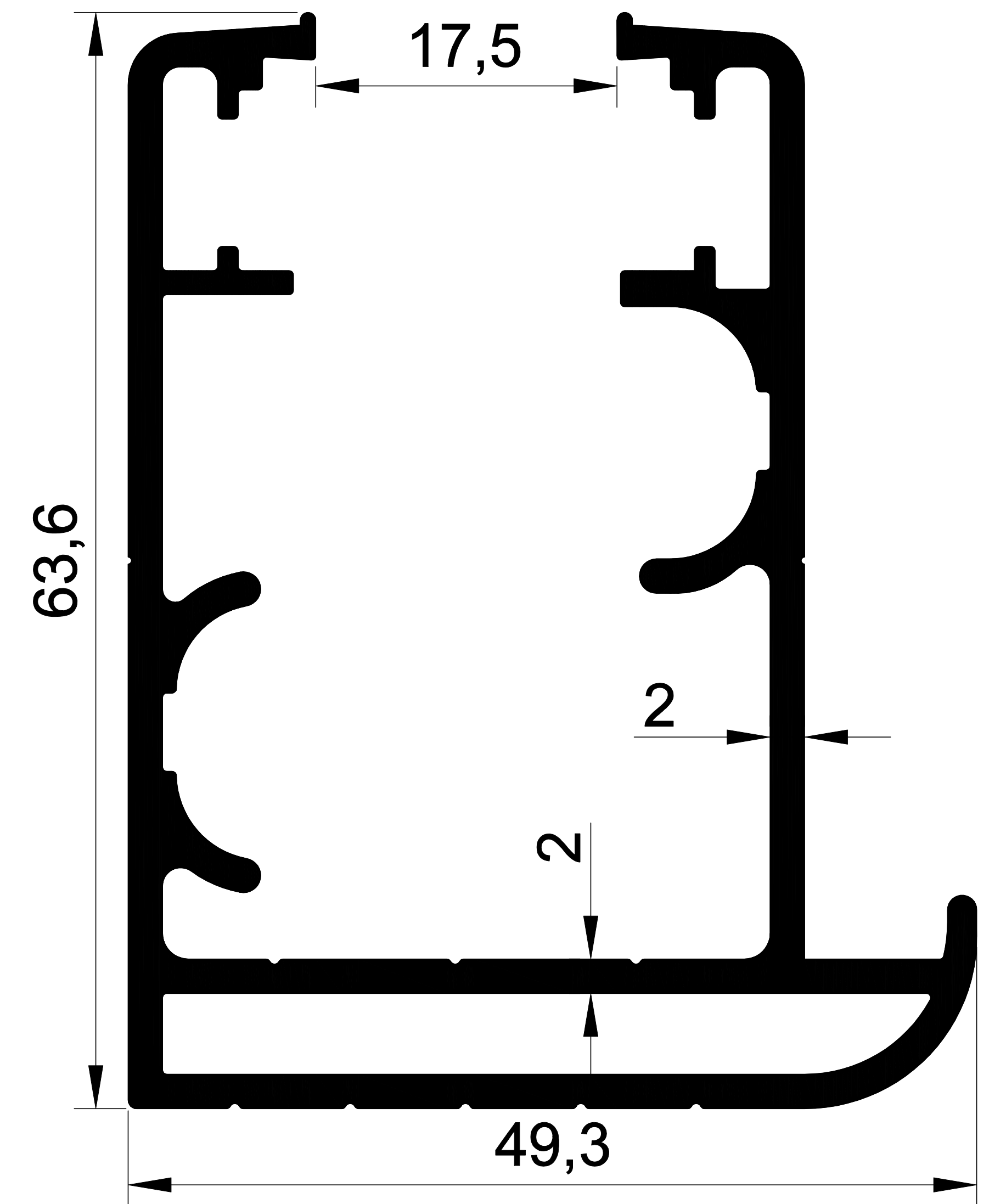
EKOL 1270 1,523 gr/m. GOLD ALTTAN DAMLALIKLI KASA
