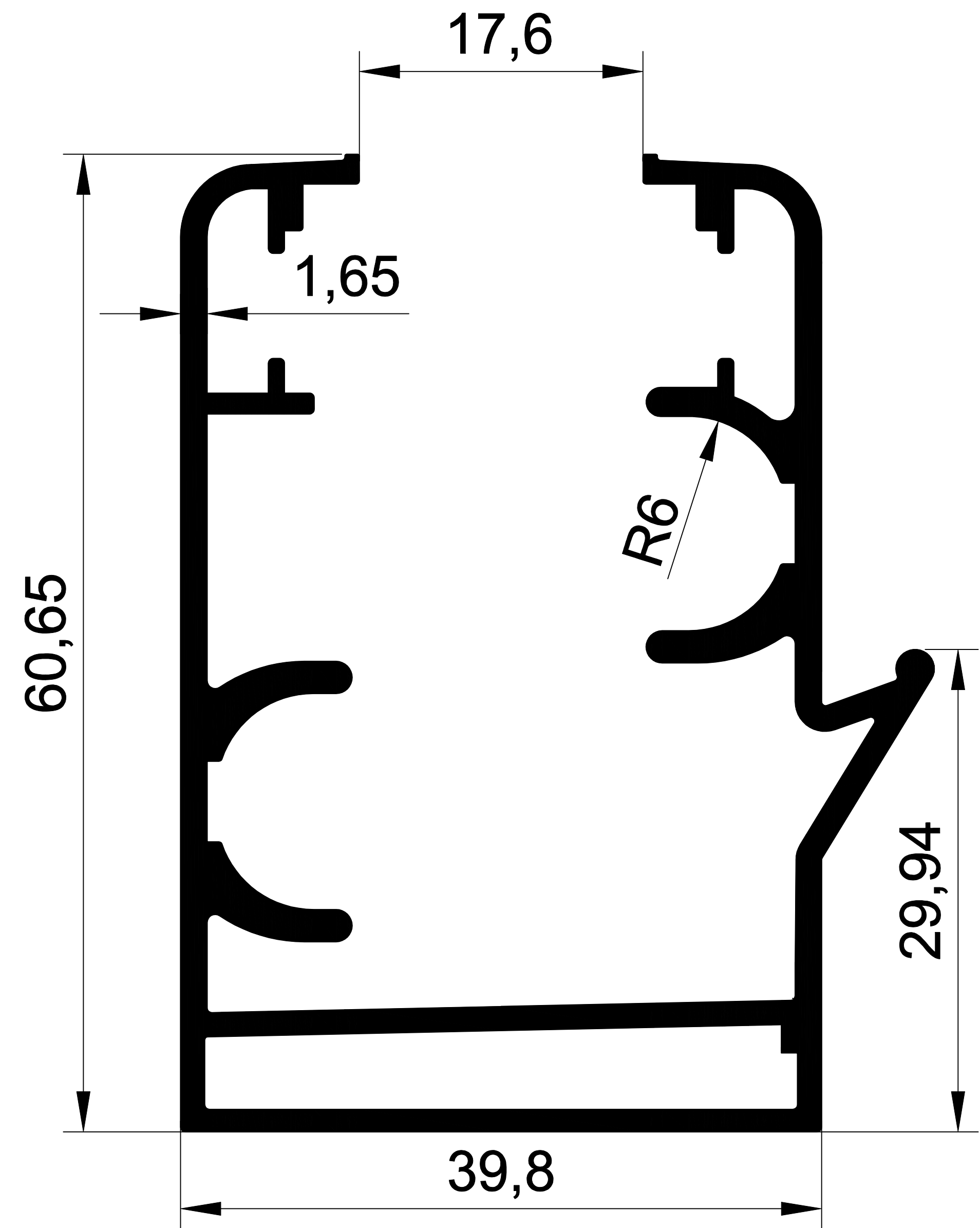
EKOL 1457 1,262 gr/m FIRTINA ORTADAN DAMLALIKLI KASA-1.6 mm
