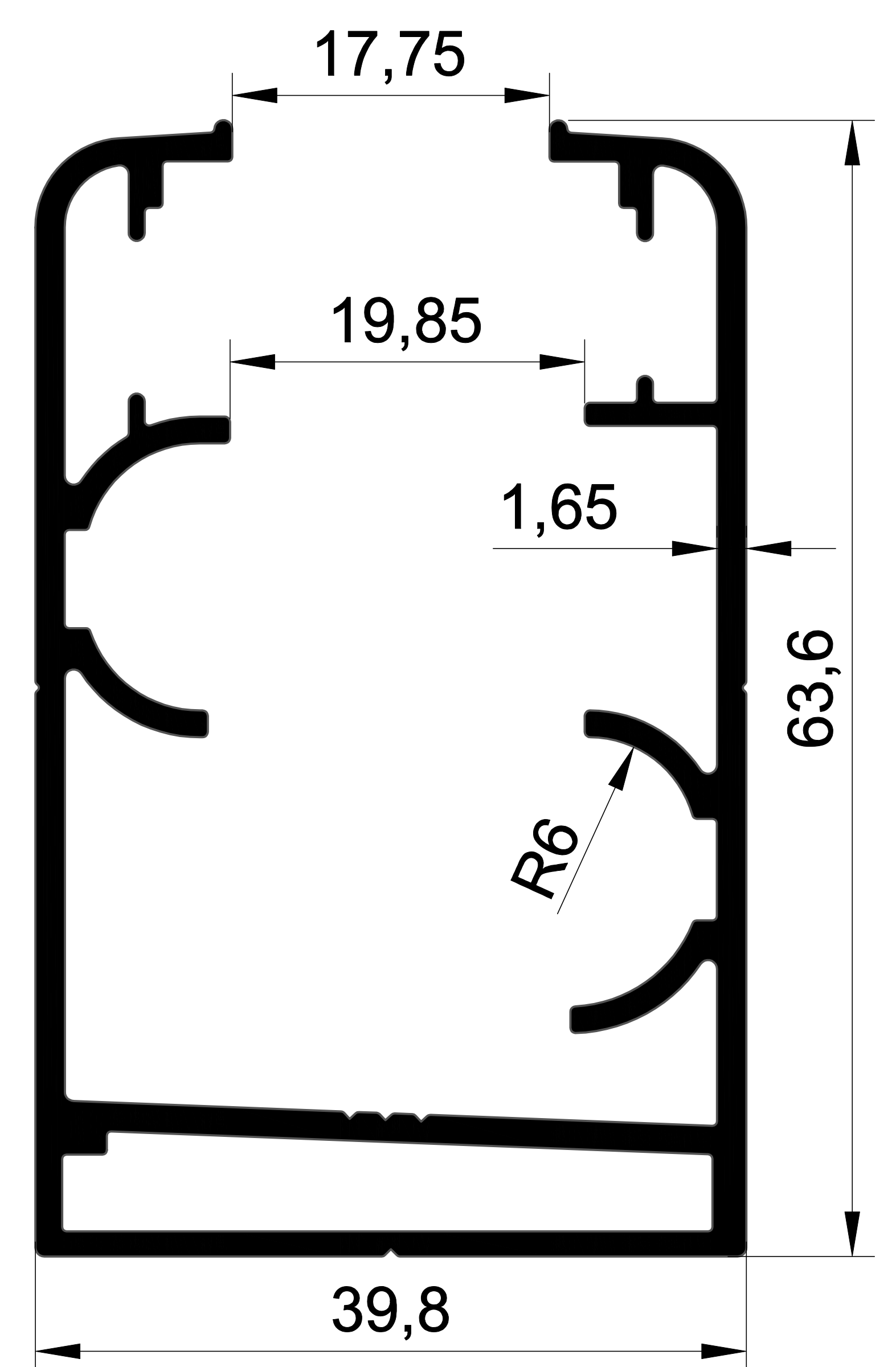
EKOL 1250-C 1,172 gr/m. GOLD KASA-1,65 mm
