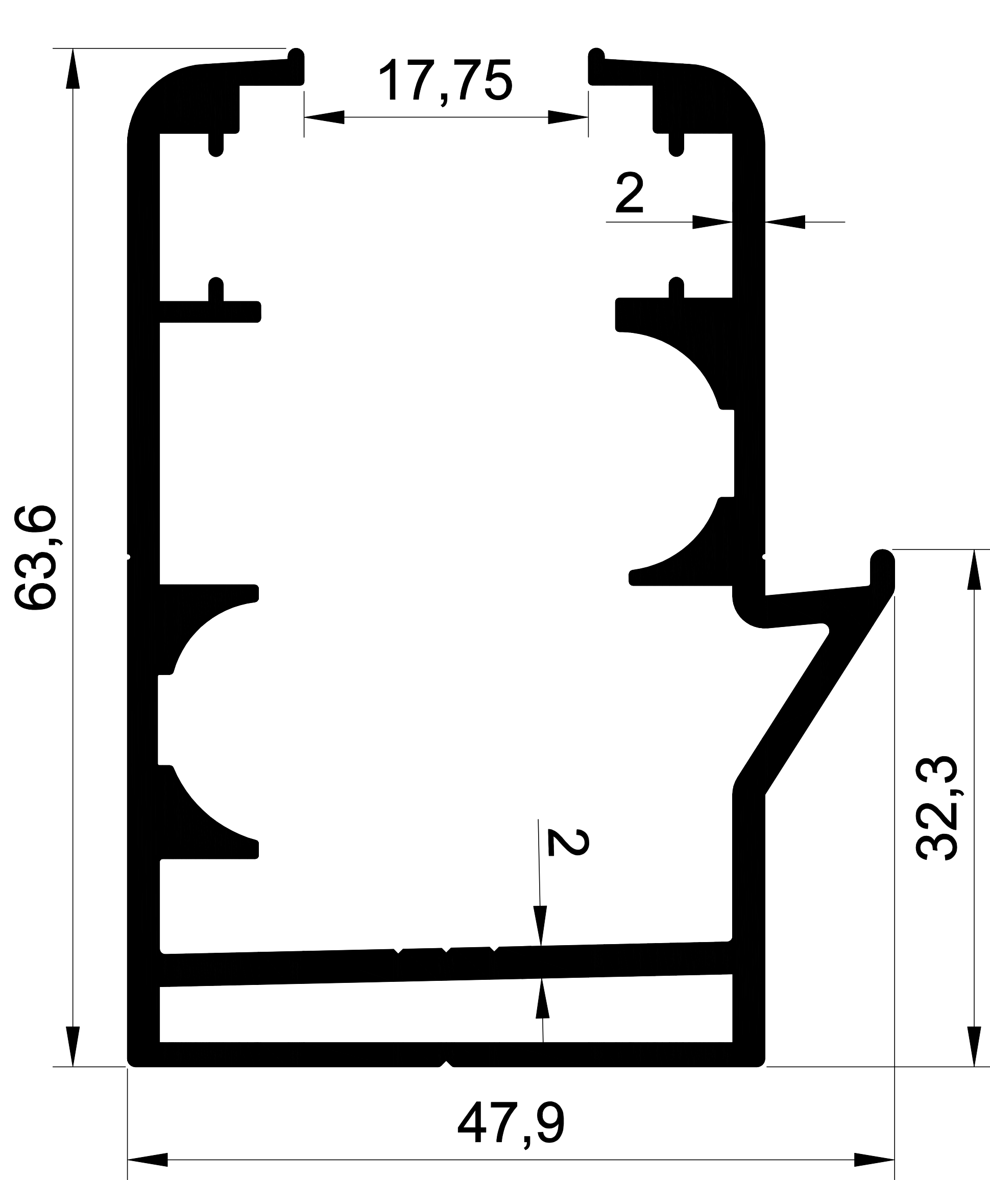
EKOL 1303 1,453 gr/m. GOLD ORTADAN DAMLALIKLI KASA
