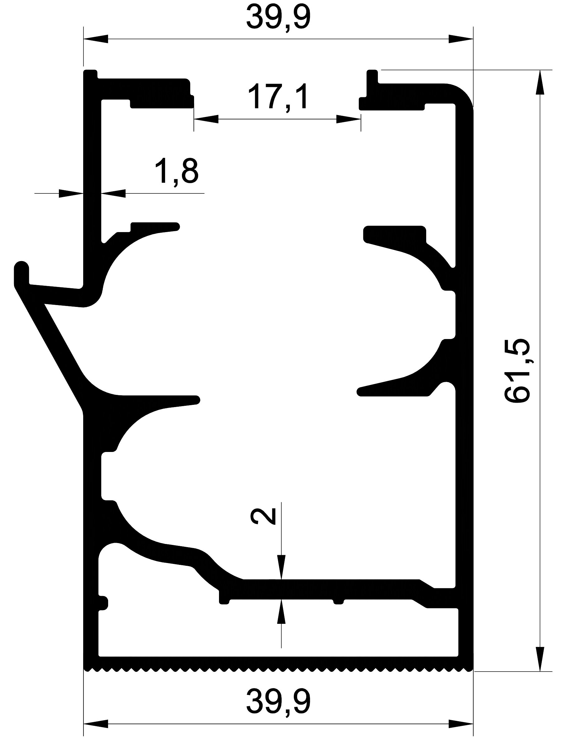
EKOL 1315 1,361 gr/m. BKS ORTADAN DAMLALIKLI KASA
